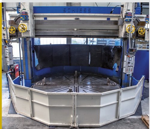
Karusselldrehmaschine SCHIESS KZ 400-450
